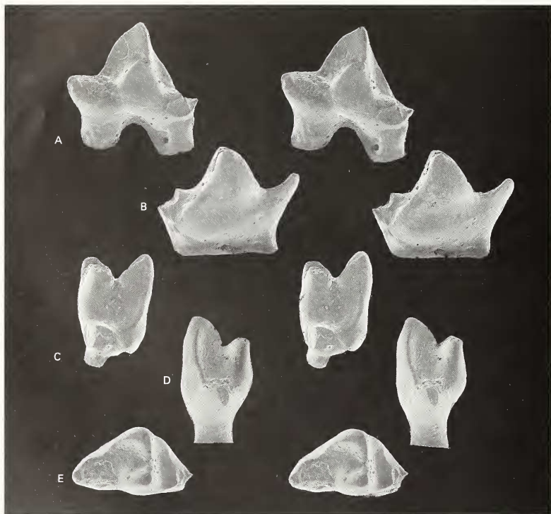
TEXT-FIG. 3. Dorsetodon haysoni gen. et sp. nov.; DORCM GS 376, resin cast; lower right molar. A, lingual view; B, labial view; C, posterior view; D, anterior view; E, occlusal view. SEM stereophotographs; \times 45 .
